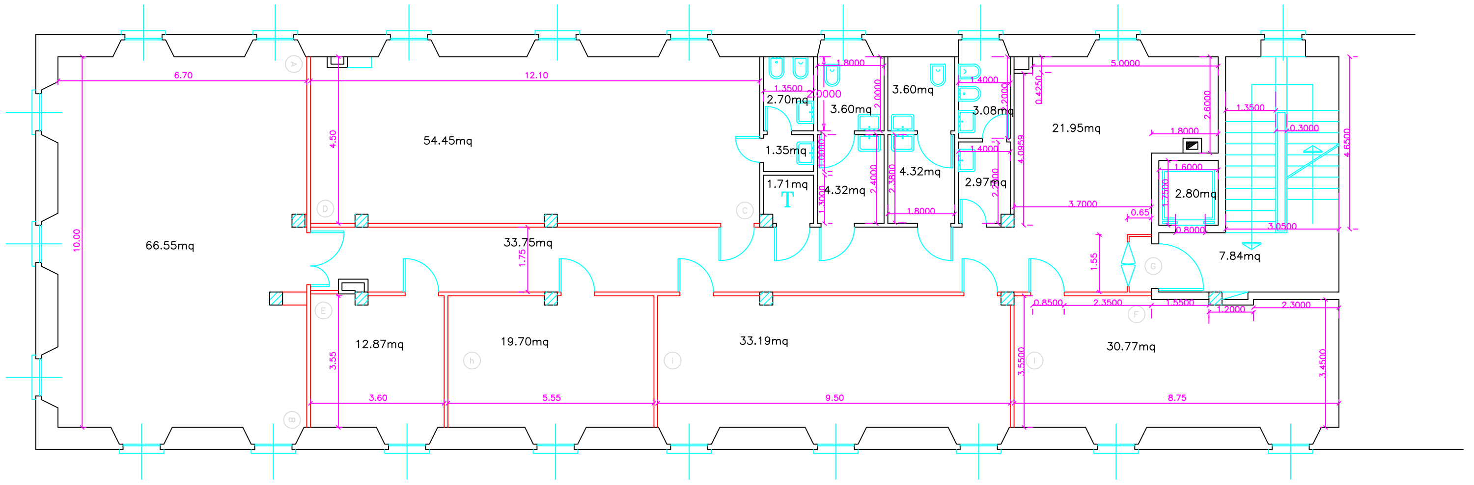
PIANTA PIANO 1*
